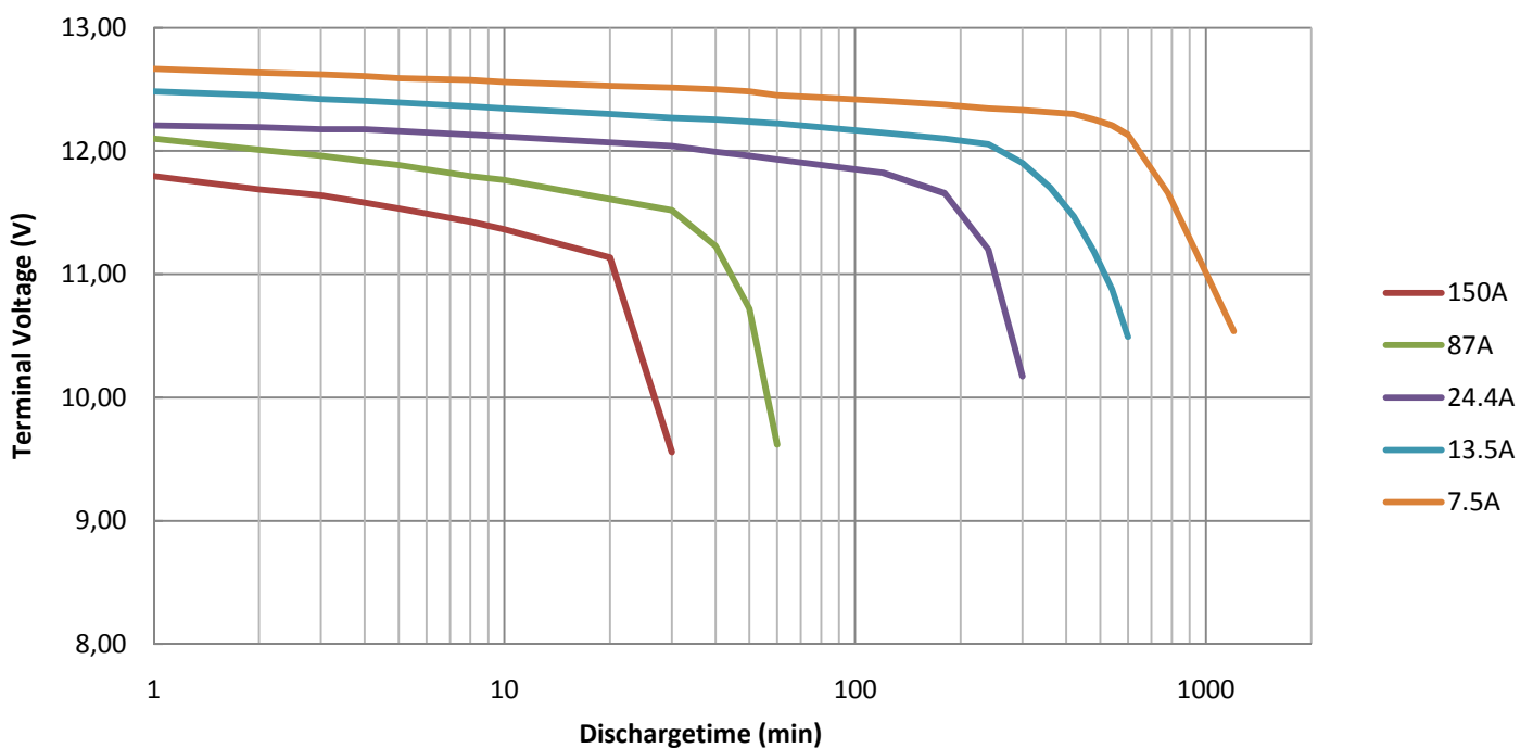
Discharge Characteristics at 25°C
