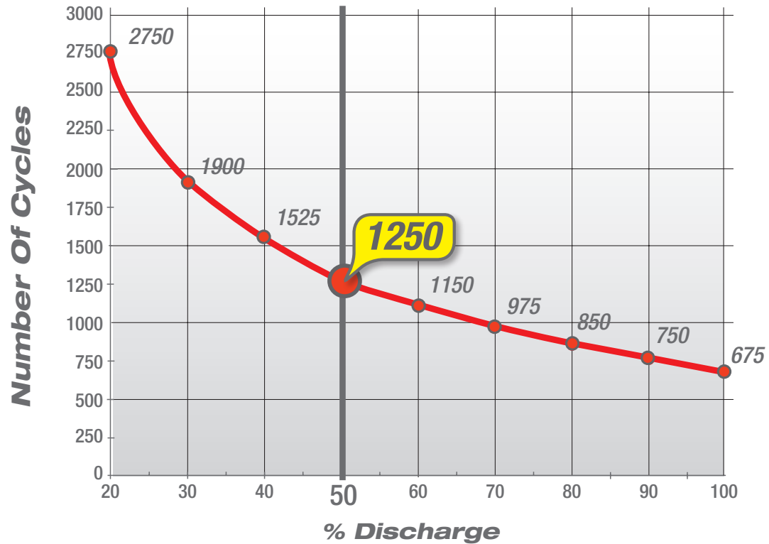
Cycle Life vs. Depth of Discharge
