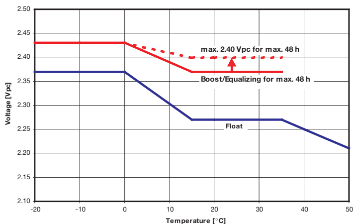
Fig. 3: A 400/FT; charging voltage vs. temperature
