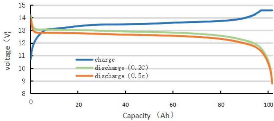
12.8V100Ah Charge-Discharge Curve (25°C)
